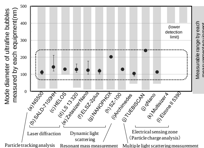
Fig. 4 Mode diameter of ultrafine bubbles measured by 6 principles of 13 equipments.
