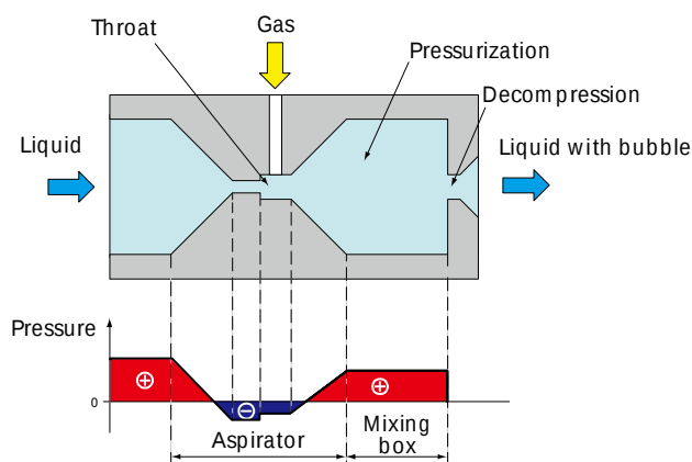
Fig.2 Schematic diagram of nanoGALF system
