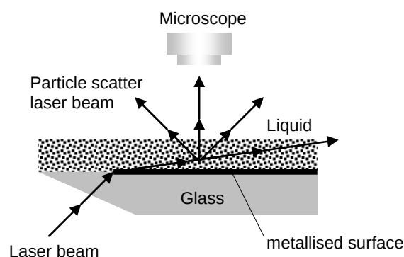
Fig.1 Principle of measurement system (LM20)
