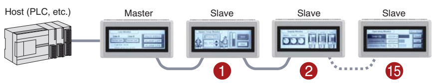
When using the HG1F RS-485/422 version as a slave, the O/I link unit is not needed.
